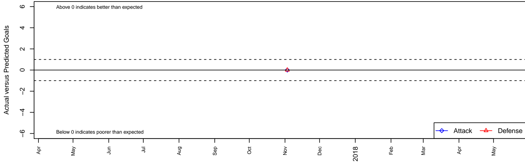
San Joaquin Valley USSDA B05 Dots are actual minus expected GF (blue circles) and GA (red triangles). Blue line is smoothed change in attack strength. Red is smoothed change in defense strength.
